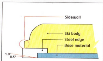
Base Edge Bevel - Usualty 0.5 to 1 degree.
